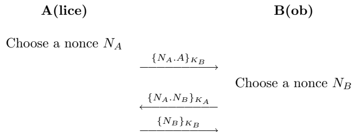
Figure 1: NSPK Protocol
